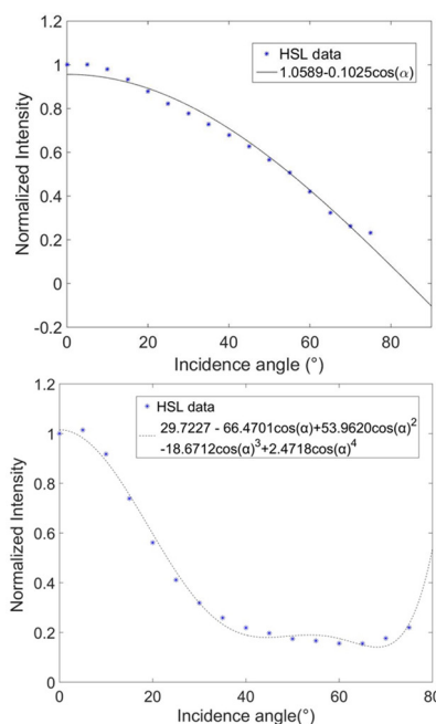
Fig. 4: Intensity normalized to 1 at 0° at 795 nm (top) and 555 nm (bottom) for the Zanzibar Gem sample (cf. Fig. 3), with the n th order cosine function (Eq. 2, with n=1 and n=4, respectively) plotted to the data.
