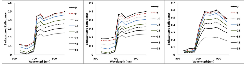
Fig. 1: Spectra vs. incidence angle. Left: Zanzibar Gem, middle: Chinese Hibiscus, right: Rose leaf.
