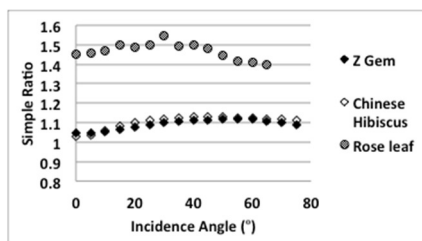
Fig. 8: The simple ratio: R760/R726 for waxed leaves, R764/713 for the rose sample.
