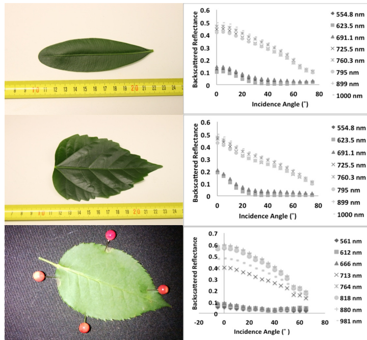
Fig. 2: The samples (left) and their incidence angle vs. backscattered reflectance (right) at all eight wavelength channels: top: Zamoculcas (Zanzibar Gem), middle: Chinese hibiscus, bottom: Rose. The pinheads are 5mm in diameter.
