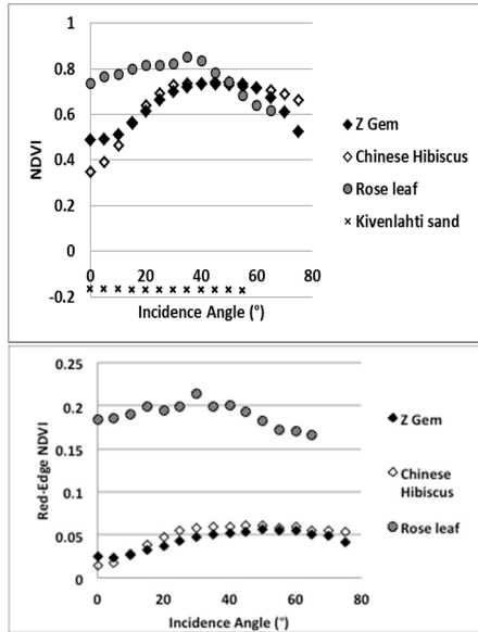
Fig. 6: Top: The NDVI index vs. incidence angle for leaf and beach sand samples. Lower: the red-edge NDVI for leaf samples.
